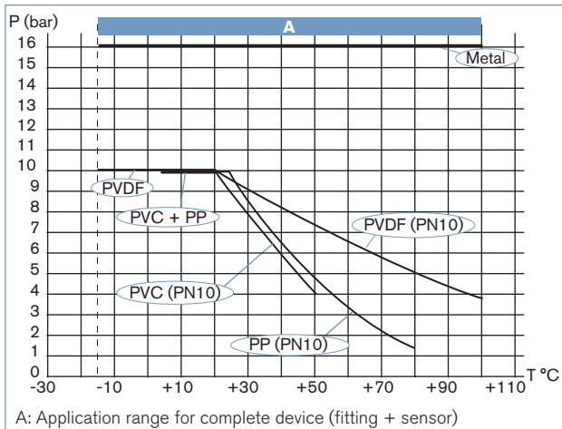
A: Application range for complete device (fitting + sensor)
